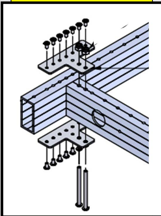
Riveted Gussets
