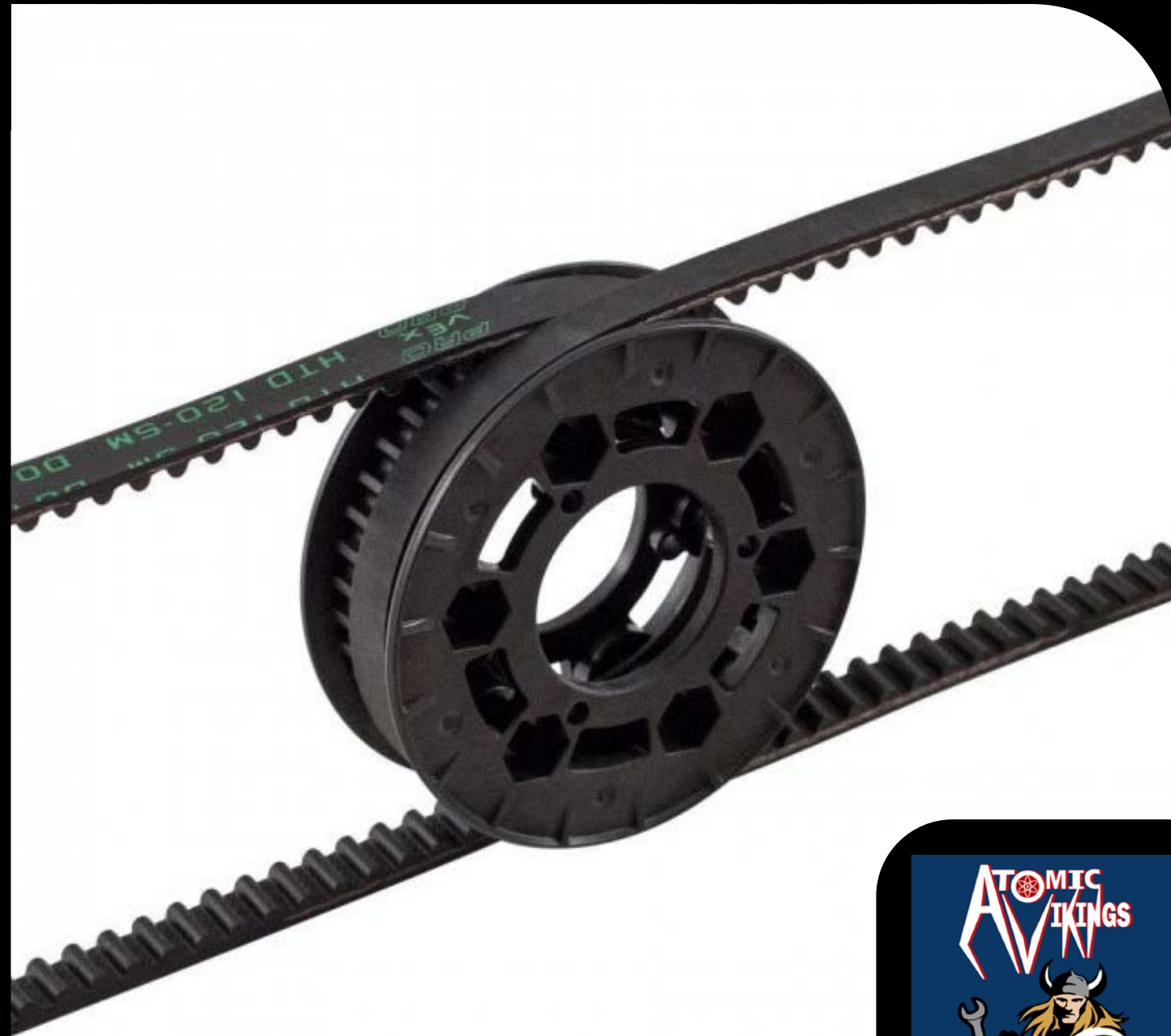
2 Vex 120 Tooth x 9mm HTD 5mm belts on a Versa pulley
