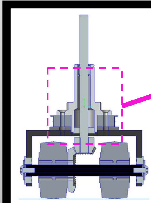
"Positraction" suspension on Team 2676's swerve drive
